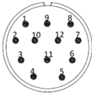
SOLDER VIEW
