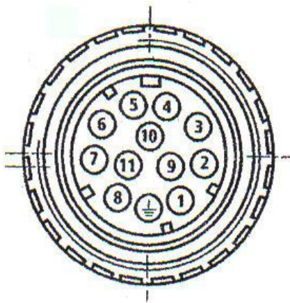
Viewed from end of connector
