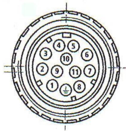
Viewed from Solder Side
